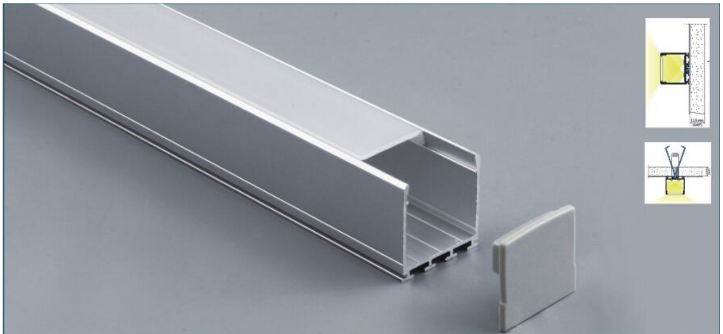
plastic end cap metal clip
