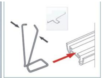
spring clip
